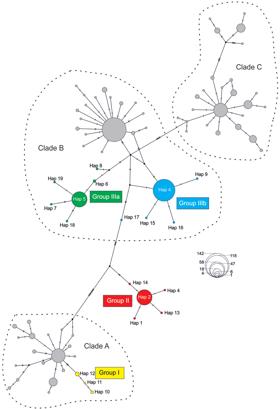
Figure 2. Median-Joining network showing phylogenetic relationships among Chinese sleeper cytochrome b haplotypes identified in our study and those (in grey) reported by Xu et al. (2014) from the native range in China. Circle size is proportional to the number of individuals with a given haplotype (see open circles with numbers).
